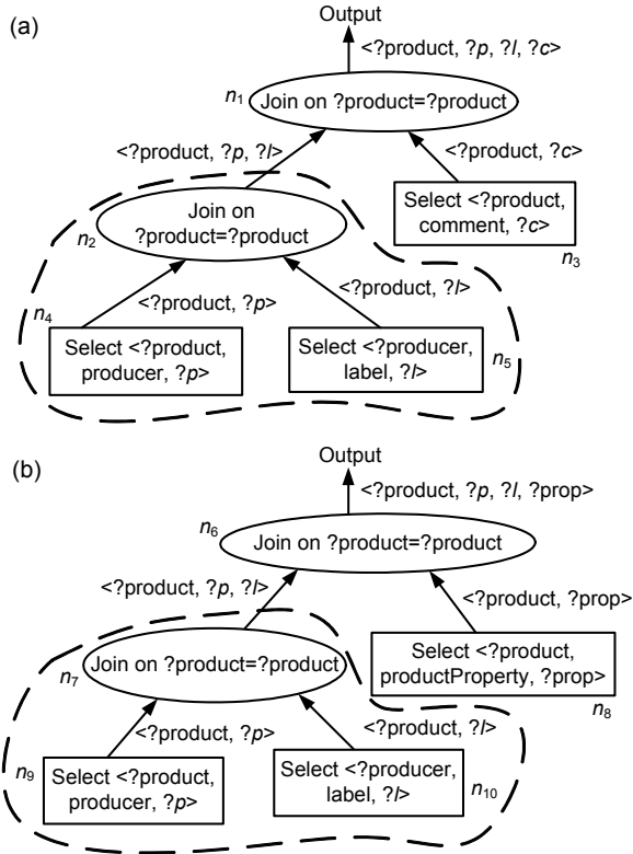
Fig. 2 Algebraic expression trees (AETs) of Query 2 (a) and Query 3 (b)
