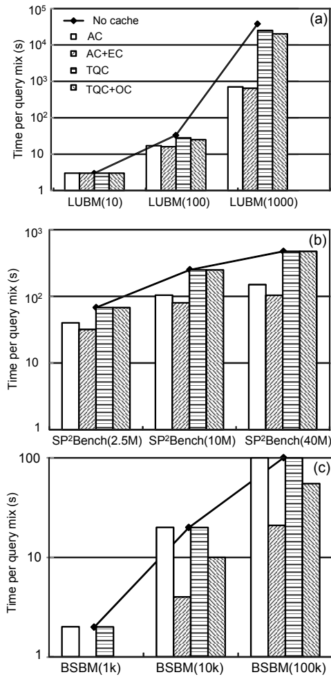
Fig. 7 Comparisons with existing approaches using datasets LUBM (a), SP 2 Bench (b), and BSBM (c)
